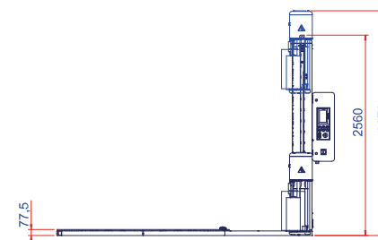
LAYOUT ROTOPLAT XL 708 PVS [mm]
