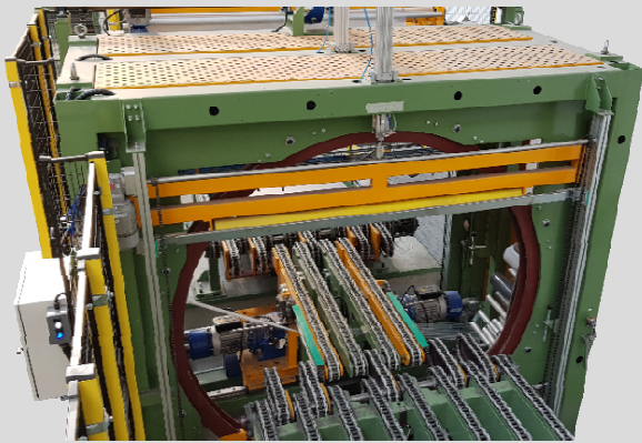
CHAINS CONVEYORS FOR STEEL SHEETS
