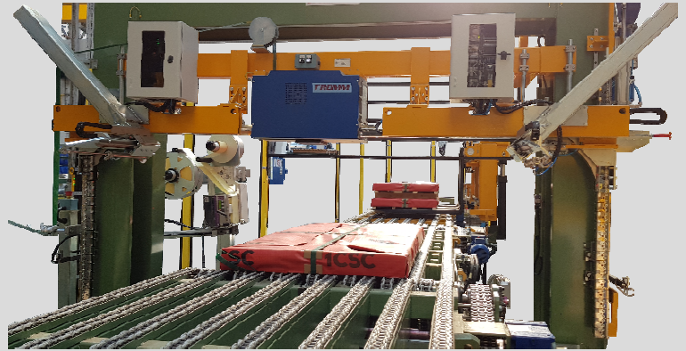
CHAINS CONVEYORS FOR STEEL SHEETS
