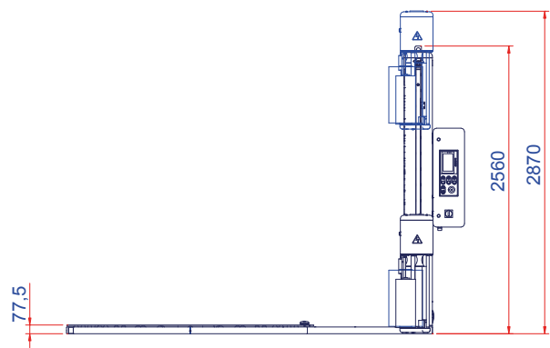
LAYOUT ROTOPLAT XL 708 PVS [mm]
