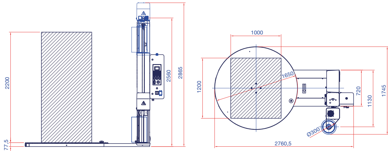
LAYOUT MASTERPLAT PLUS PGS [mm]
